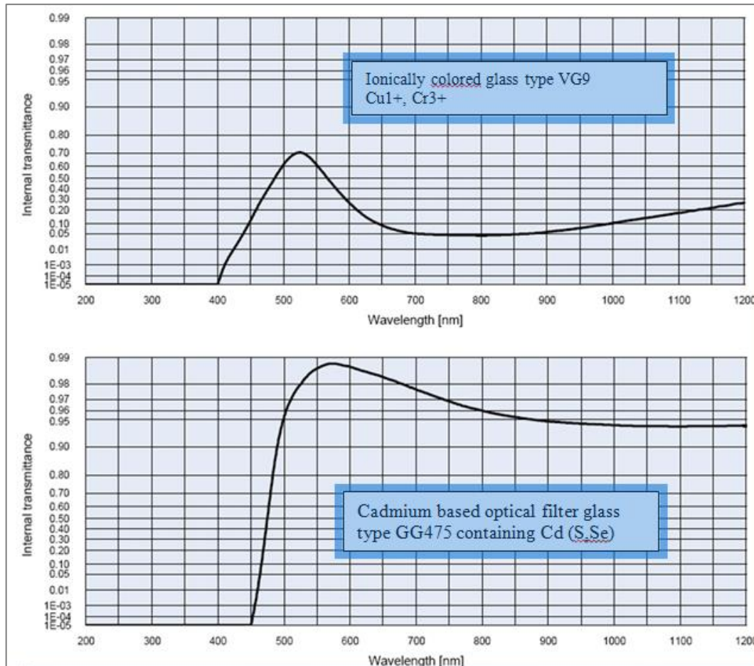
Figure 8-3: Spectra Comparison: Ionically Coloured Glass (above) Cd Glass (below)
